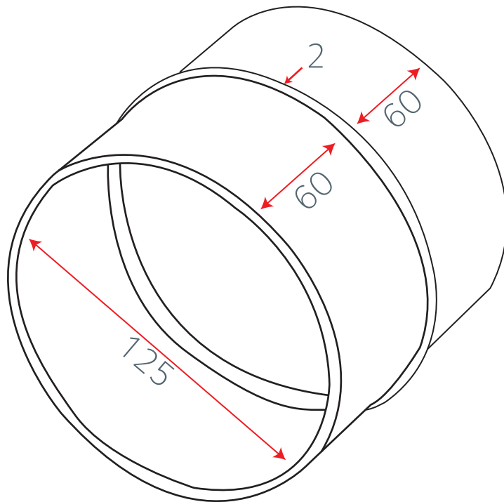
5" - 150 x 70 Ducting
