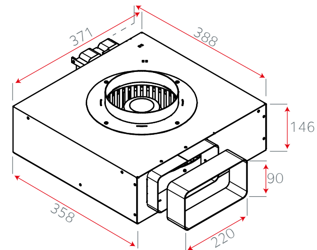
Motor Unit
