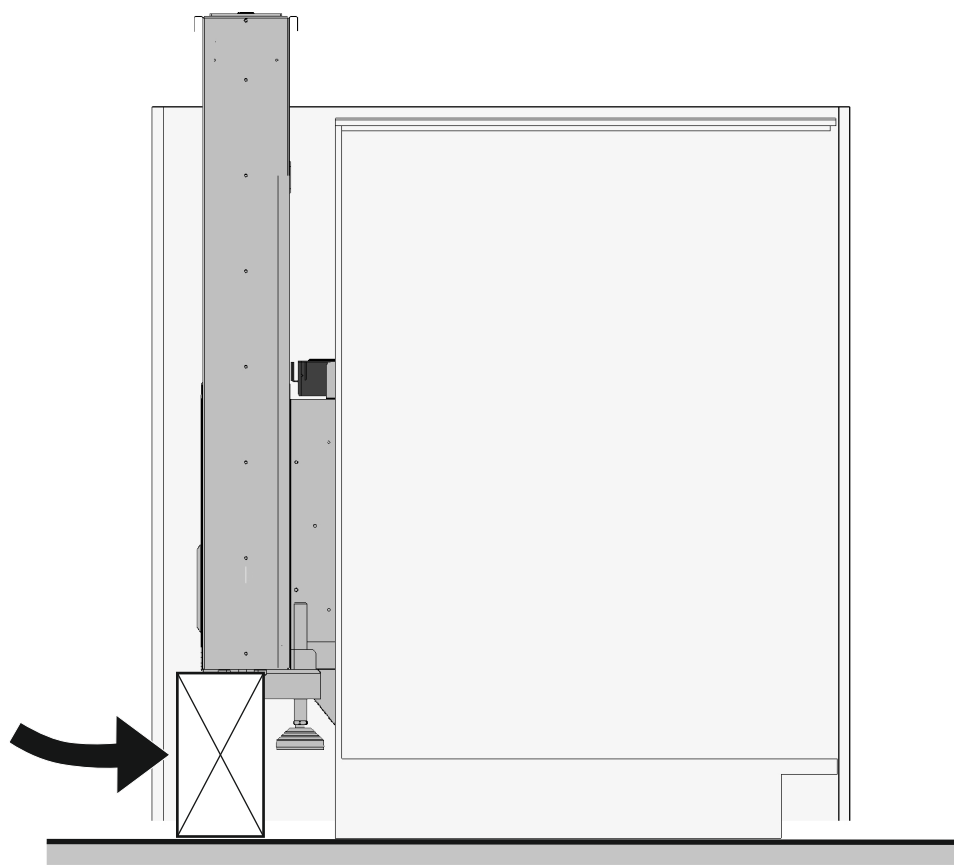
SUSPENSION BLOCK
