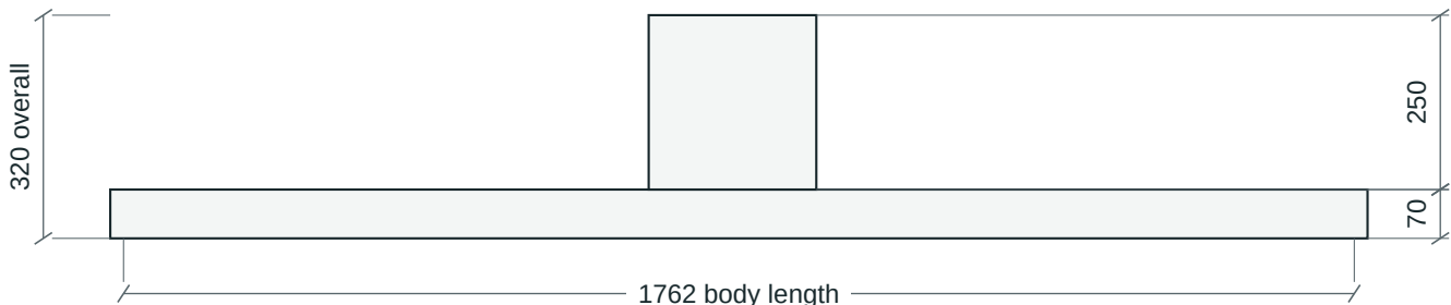
Motor position shown schematically; adjustable outlet orientation.
